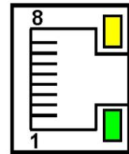
Fig.19. View and numbering of RJ45 slot pins
