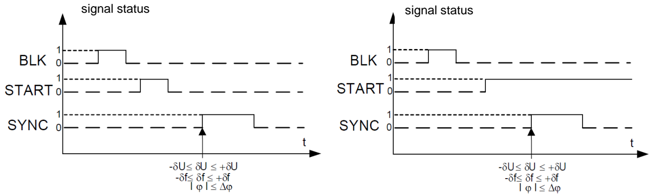
a,b) SYNC relay energized after synchronization conditions are met
